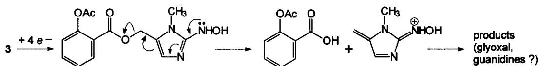
Scheme 3. Proposed mechanism for the reductive elimination of aspirin from 3 .
