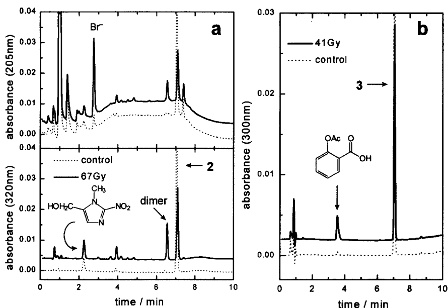
Figure 1. Product profiles obtained on reduction of 2 (a) and 3 (b).
